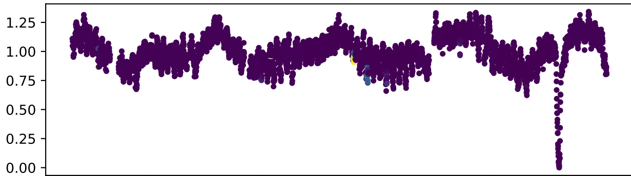
Single Model Predictions - KIC 3542116
