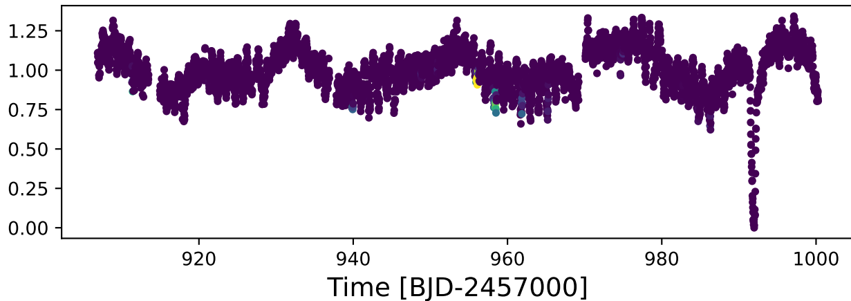
Single Model Predictions - KIC 3542116
